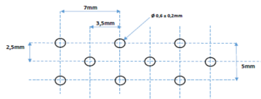
P31 perforation: 0,6 ± 0,2mm holes
